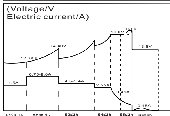
Charging characteristic
